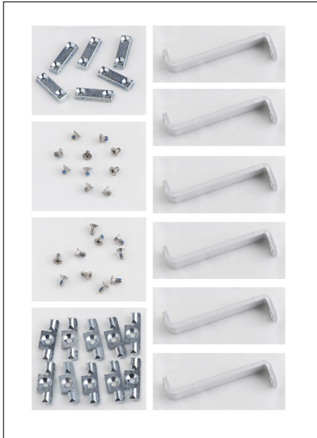
34194A dual lock link kit: recommended for side-by-side combinations and includes links for instruments of different depths. This kit can be used with the 34191A 2U dual flange kit to mount two half-width, 2U height instruments side-by-side.
